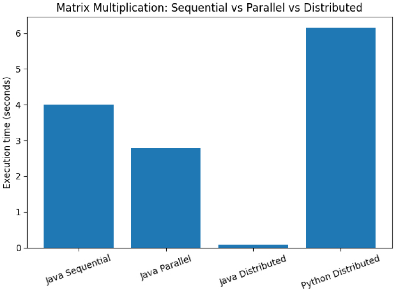
Figure 1: Execution time comparison: Java sequential, Java parallel, Java distributed and Python distributed matrix multiplication (matrix size 500 \times 500 , 4 workers).
